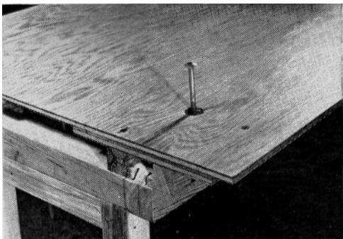
This 1/2" bolt is a lock to keep table from sliding off when in storage position. Use a bolt long enough to be tapped up from the bottom for removal.
