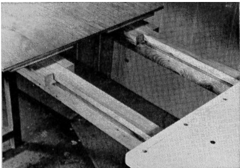
Guide-slide assembly should be positioned accurately, dressed for loose fit so table moves easily. This one is built-up 3/8" ply; 3/4" would be better.
