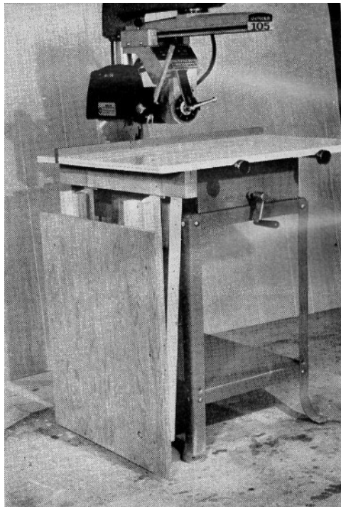
In storage position, extension table rests within floor space required by tool alone. Saw make and pedestal determine attachment-block location.
